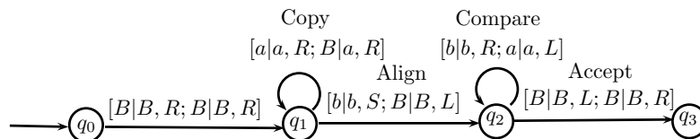
Figure 4.2: Recognition of language L = \{a^n b^n \mid n \geq 0\} using a two-tape TM.
